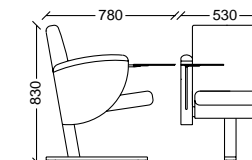
Posto panca mobile sedile e schienale quadro fianco sospeso con tavoletta Square seat and backrest suspended and mobile bench with writing board
