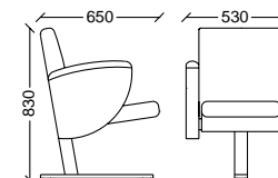
Posto panca mobile sedile e schienale quadro fianco sospeso Square seat and backrest mobile bench with suspended side
