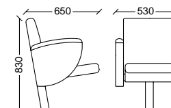
Schienale quadro fianco sospeso Square backrest on the suspended bench side
