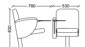
Panca mobile sedile e schienale arrotondato fianco sospeso con tavoletta Round seat and backrest suspended and mobile bench with writing board
