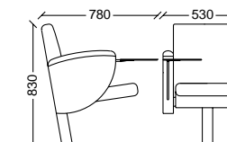
Schienale quadro fianco sospeso con tavoletta Square backrest on the suspended bench side with writing board
