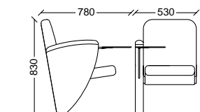
Schienale e schienale arrotondato fianco a pavimento con tavoletta Round backrest and seat on the bench side fixed to the floor with writing board
