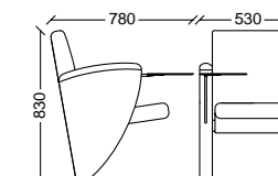
Sedile e schienale quadro fianco a pavimento con tavoletta Square backrest and seat on the bench side fixed to the floor with writing board
